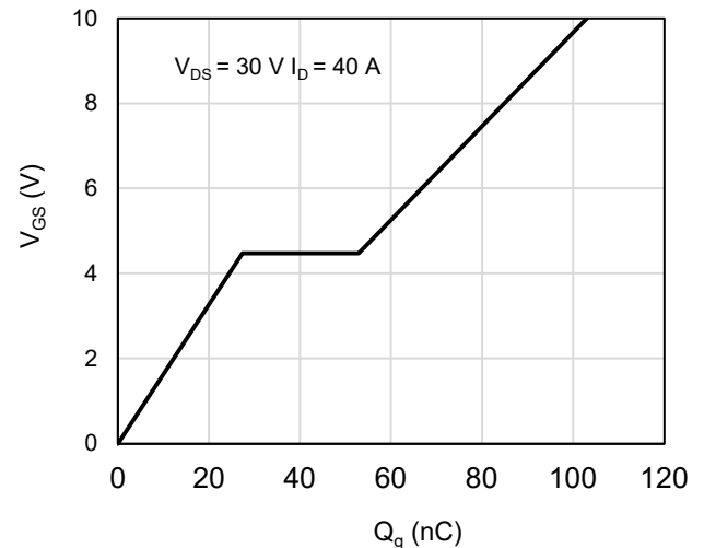
Figure 10: Gate-Charge Characteristics
